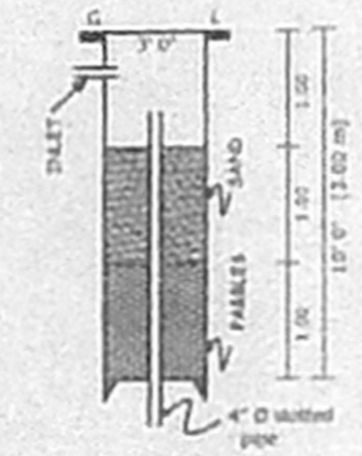
RAIN WATER PERCOLATION PIT SCALE 1:75
