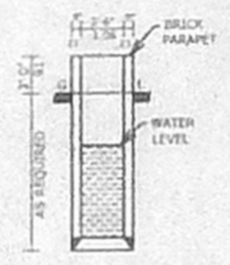
SECTION OF WELL SCALE 1:75
